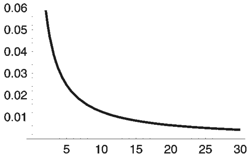
FIG. 4. Percentage error in the one term asymptotic expansion of the Hankel function.
