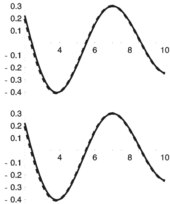
FIG. 3. Exact solution (solid curve) and asymptotic expansion (dashed curve) of the real part (upper plot) and imaginary part (lower plot) of the Hankel function starting at \lambda = 2 .
