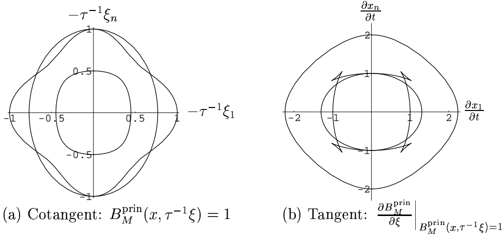
Figure 1: (a) Section of a slowness surface (the characteristic surface) for a transversely isotropic medium in n = 3 dimensions. (b) Set of velocities associated to the slowness surface in a). Note the caustics that occur due to the fact that one of the sheets is not convex.
