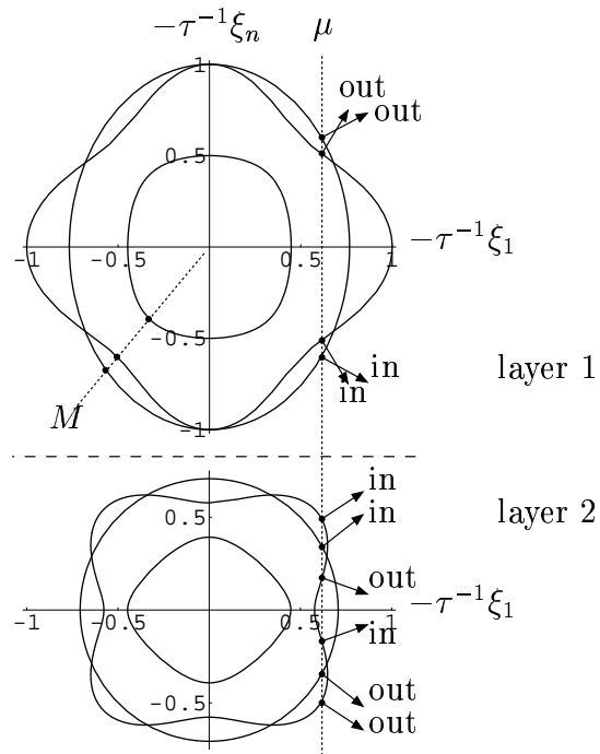
Figure 3: 2-dimensional section of an n = 3 -dimensional slowness surfaces at some point of the interface, for the medium on both sides of the interface. The slownesses of the modes that interact (i.e. reflect and transmit into each other) are the intersection points with a line that is parallel to the normal of the interface. The group velocity, which is normal to the slowness surface, determines whether the mode is incoming or outgoing.
