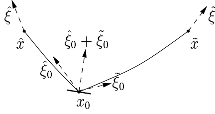
Figure 4: The scattering cotangent vectors.
