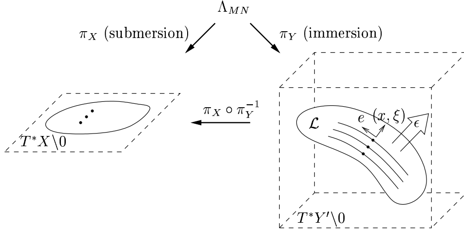
Figure 5: Visualization of the symplectic structure of \Lambda_{MN} (cone structure omitted).
