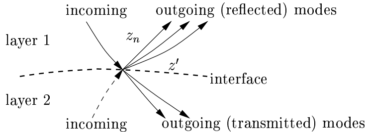
Figure 2: Incoming and outgoing rays
