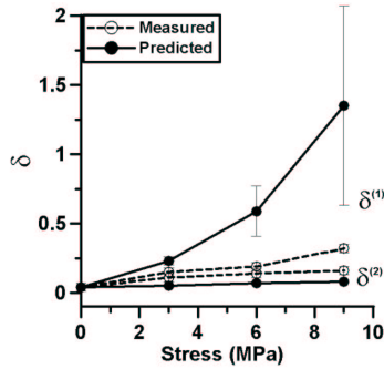
Fig. 5: Measured and predicted \delta^{(1)} and \delta^{(2)} versus applied uniaxial stress. Stress was applied in the x_2 direction.
