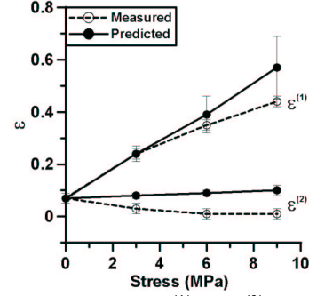
Fig. 3: Measured and predicted \epsilon^{(1)} and \epsilon^{(2)} versus applied uniaxial stress. Stress was applied in the x_2 -direction.
