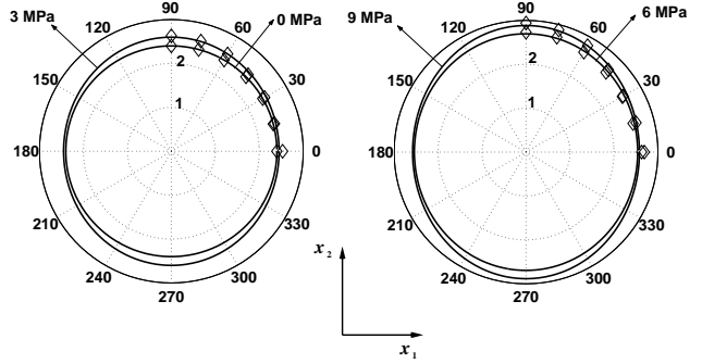
Fig. 2: Moveout velocities (km/s) of P -wave (diamonds) obtained by semblance analysis at different azimuths and stress levels. The best-fit NMO ellipses are also shown. Stress was applied in the direction of x_2 -axis ( 90^\circ ).
