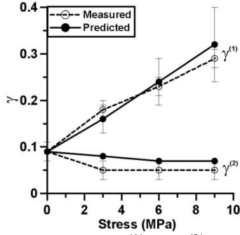
Fig. 4: Measured and predicted \gamma^{(1)} and \gamma^{(2)} versus applied uniaxial stress. Stress was applied in the x_2 -direction.
