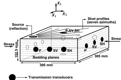
Fig. 1: Schematic drawing of the experiment performed on the block of Berea sandstone under several uniaxial stresses. Transmission velocities were measured by transducers, shown here as dark solid circles. Multi-azimuth acquisition of PP and PS reflection data was conducted on the top of the block.
