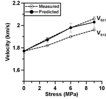
Fig. 6: Measured and predicted V_{S12} and V_{S21} velocities versus applied uniaxial stress. Stress was applied in the x_2 direction.
