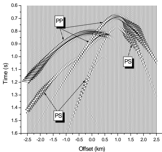
Figure 6: Seismogram computed with ERC.
