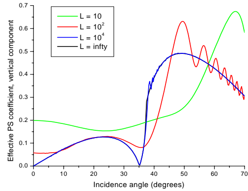
Figure 4: Absolute value of the PS ERC.
