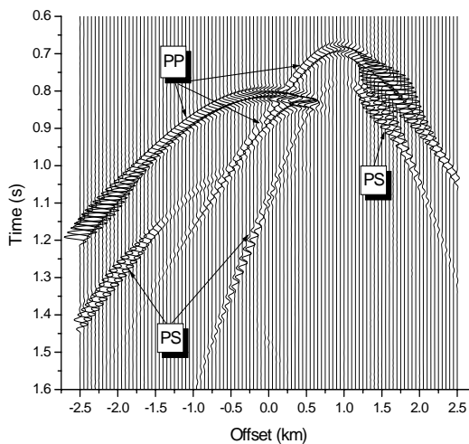
Figure 6: Seismogram computed with ERC.
