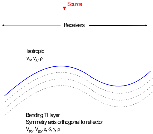
Figure 1: In-line section of the model.
