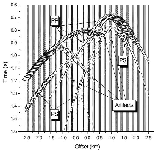
Figure 5: Seismogram computed with PWRC.
