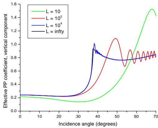
Figure 3: Absolute value of the PP ERC.
