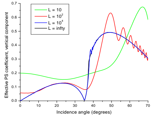
Figure 4: Absolute value of the PS ERC.
