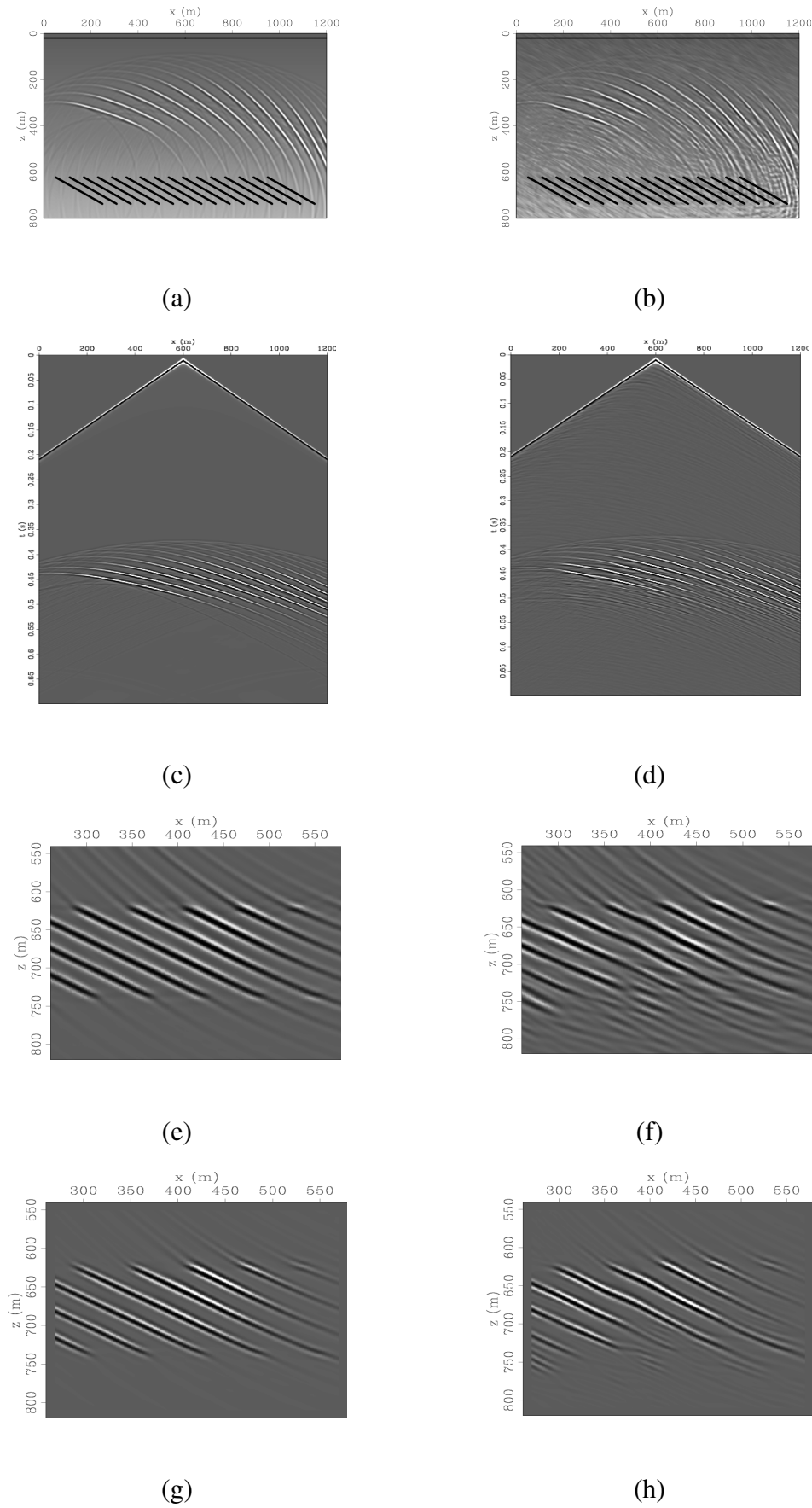
Figure 1: Velocity models and simulated wavefields (a)-(b), recorded data (c)-(d), migration with Conventional IC (e)-(f), and with Interferometric IC (g)-(h).
